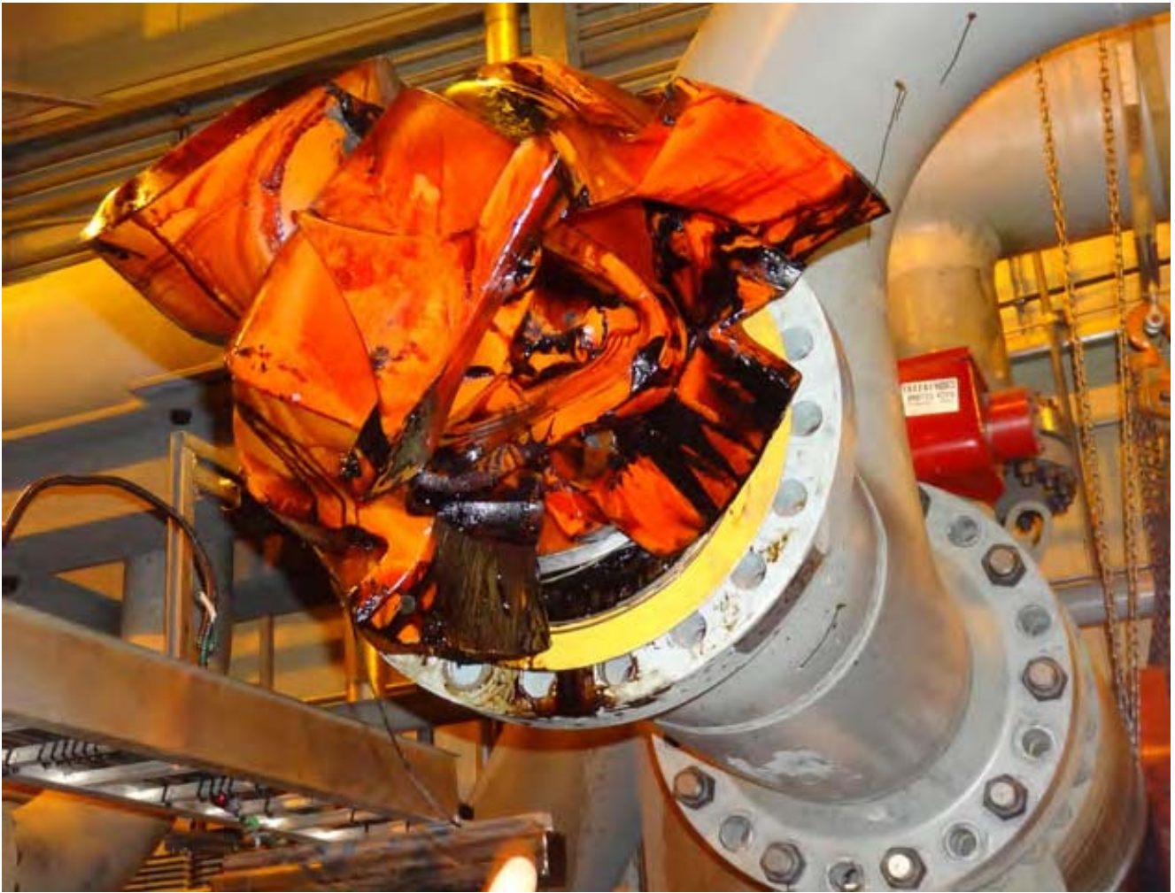
Damaged scraper pig lodged in discharge pressure relief piping at PS5 (photo courtesy of BLM).
